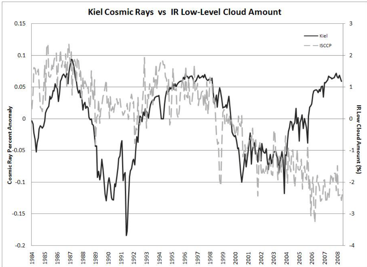
Figure 2. Surface-based neutron counter at Kiel, Germany, depicting cosmic ray percentage anomaly versus the ISCCP lower troposphere global cloudiness. The Kiel Neutron Monitor is located at 54°N and 10°E, at an altitude of 54m above sea level, with a geomagnetic cutoff rigidity of 2.32 GV. (Please note that the Beijing GCR record is very similar to the Kiel plot shown above.)
